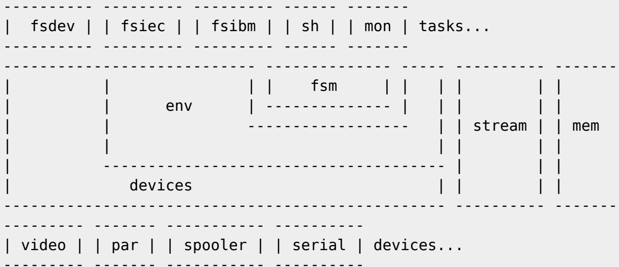
Fig.1: General OS structure. The devices and tasks make up the features of the system, while the kernel provides communications. (fsm = filesystem manager, env = environment handling, task switcher)
